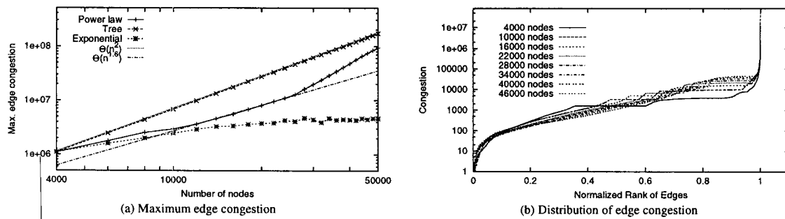
Figure 5: Edge congestion with shortest path routing and any-2-any communication: The figure on the left shows the maximum edge congestion. The figure on the right shows the distribution of congestion over all links, with the number of links normalized to 1 in each case. The figure on the left also plots the worst congestion for exponential graphs and preferential connectivity trees.
