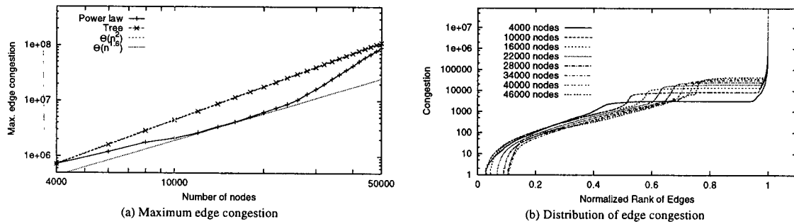
Figure 6: Edge congestion with shortest path routing and leaf-2-leaf communication
